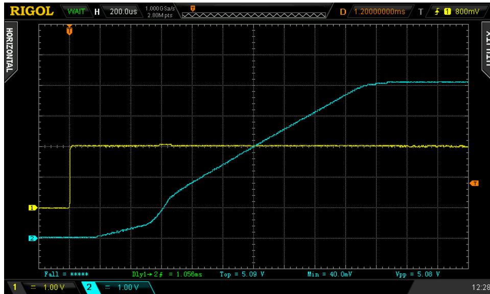
Figure 2. A SLG59M1710V with C_{SLEW} set to 4nF and 470μF for C_{LOAD} . C_{LOAD} -to- C_{SLEW} ratio is greater than 33,600. Note that the internal SCL monitor's been triggered and V_{OUT(SR)} is reduced until V_{OUT} reaches ~0.3V.
