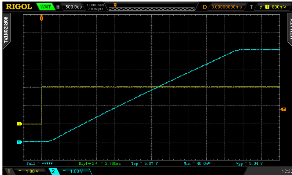
Figure 3. A SLG59M1710V with C_{SLEW} set to 15nF and 470μF retained for C_{LOAD} . C_{LOAD} -to- C_{SLEW} ratio is smaller than 33,600. Note smooth V_{OUT} transition.
